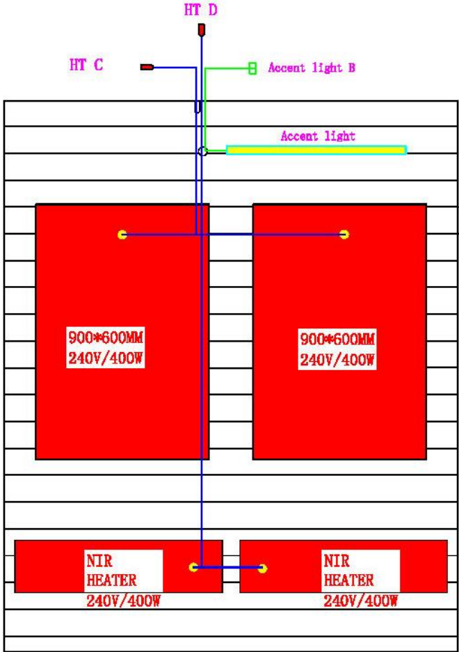
Rear wall panel
