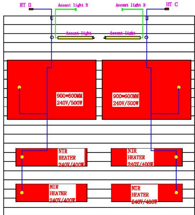
Rear wall panel
