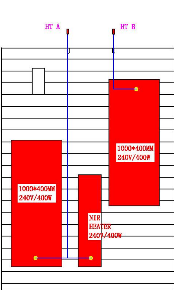
left side wall panel
