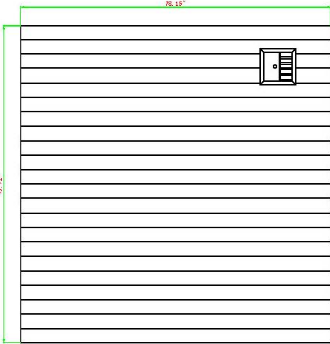
left side wall panel
